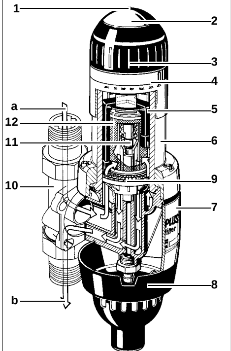
Fig. 7: Functional description
