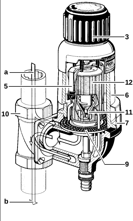
Fig. 7: Functional description
